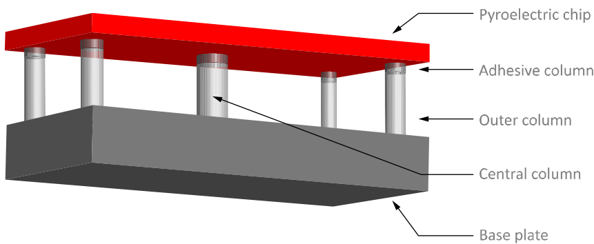
Figure 27: Chip holder for reducing the microphonic effect, design model from FEM simulation
