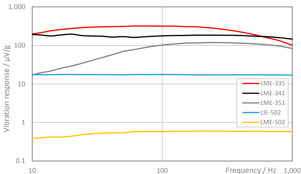
Figure 30: Measurement results of the vibration response across the mechanical excitation frequency:
