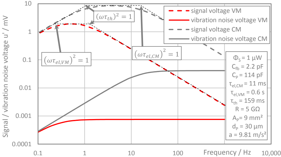
Figure 29: Comparison of desired signal and vibration noise voltage in voltage mode (VM) and current mode (CM)
