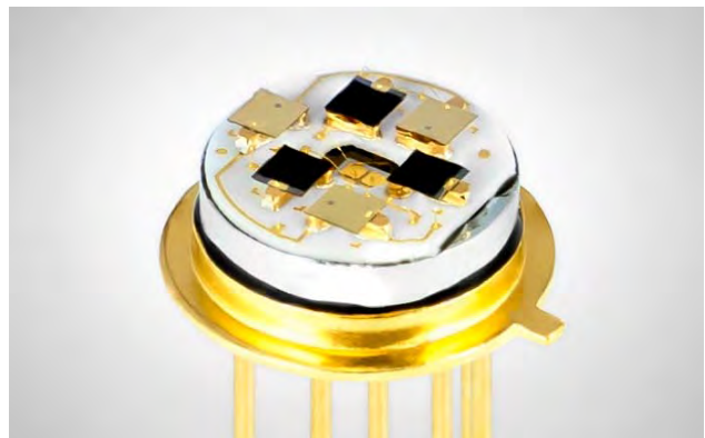
Figure 14: Additional chips for thermal compensation (without black absorbing layer)
