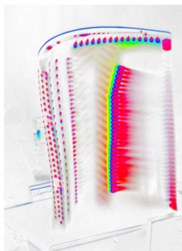
Thermographic testing of turbine blades
