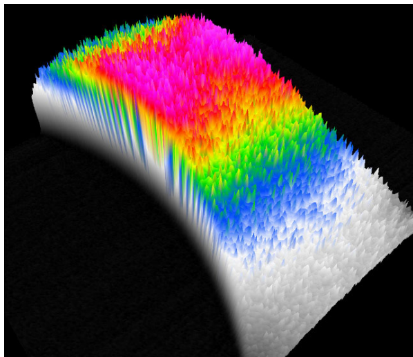
Fig. 4-6: Lock-In amplitude result of sample 2 at the start of the load cycle. A relatively symmetrical temperature (stress) distribution can be recognised over the sample cross-section. At the bottom left the 3D visualization is shown with the same scaling.
